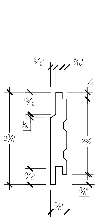
COUPE - 1"X4"
