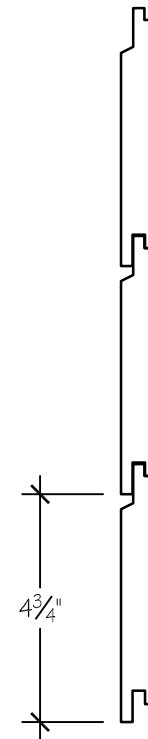
COUVRANT 1"X6"
