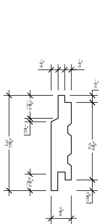
COUPE - 1"X4"
